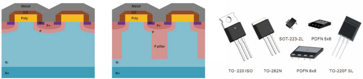
Figure 1 Device structure: SJ-MOS VS VDMOS
